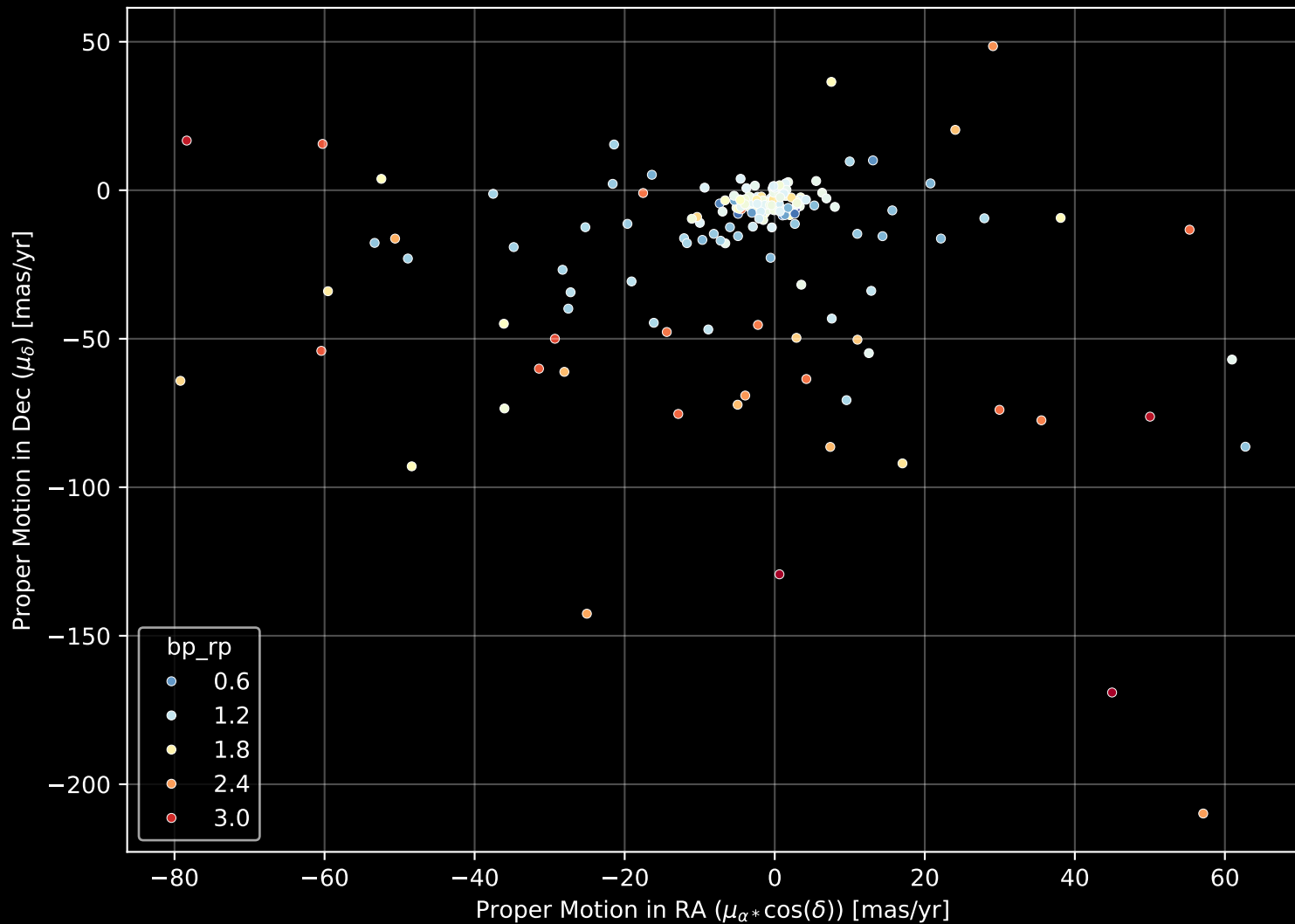
APOGEE DR17 Field: [K2_C7_010-14_btx] Proper Motion Diagram (n= 183)
