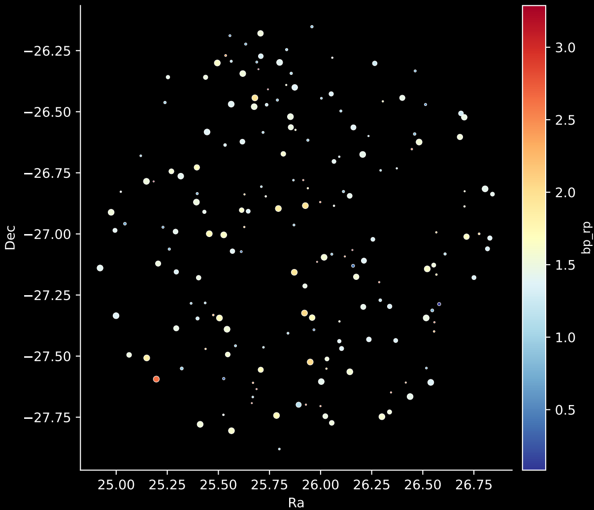
APOGEE DR17 Field: [K2_C7_010-14_btx] Stars: 183
