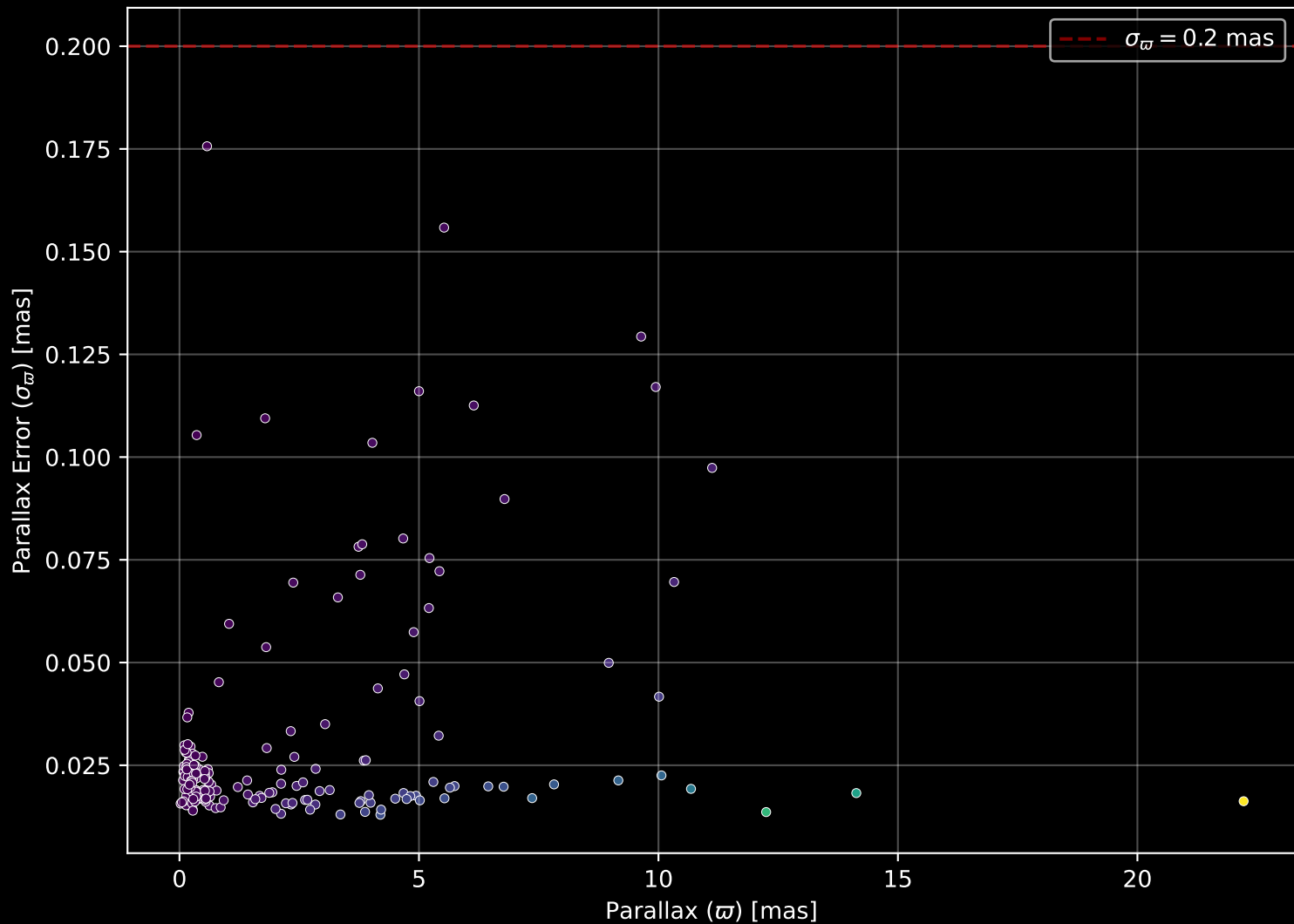
APOGEE DR17 Field: [K2_C7_010-14_btx] Parallax Quality (n= 183)
