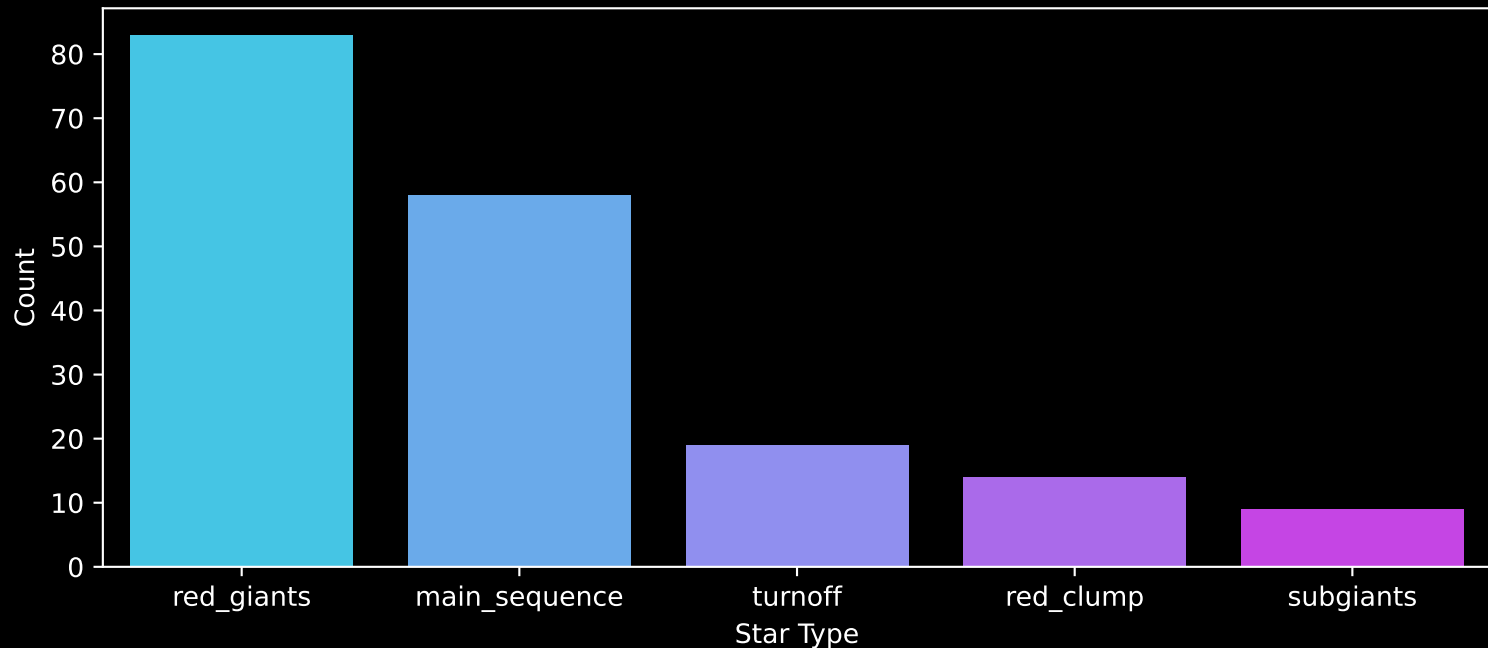
APOGEE DR17 Field: [K2_C7_010-14_btx] Count plot of Star Type
