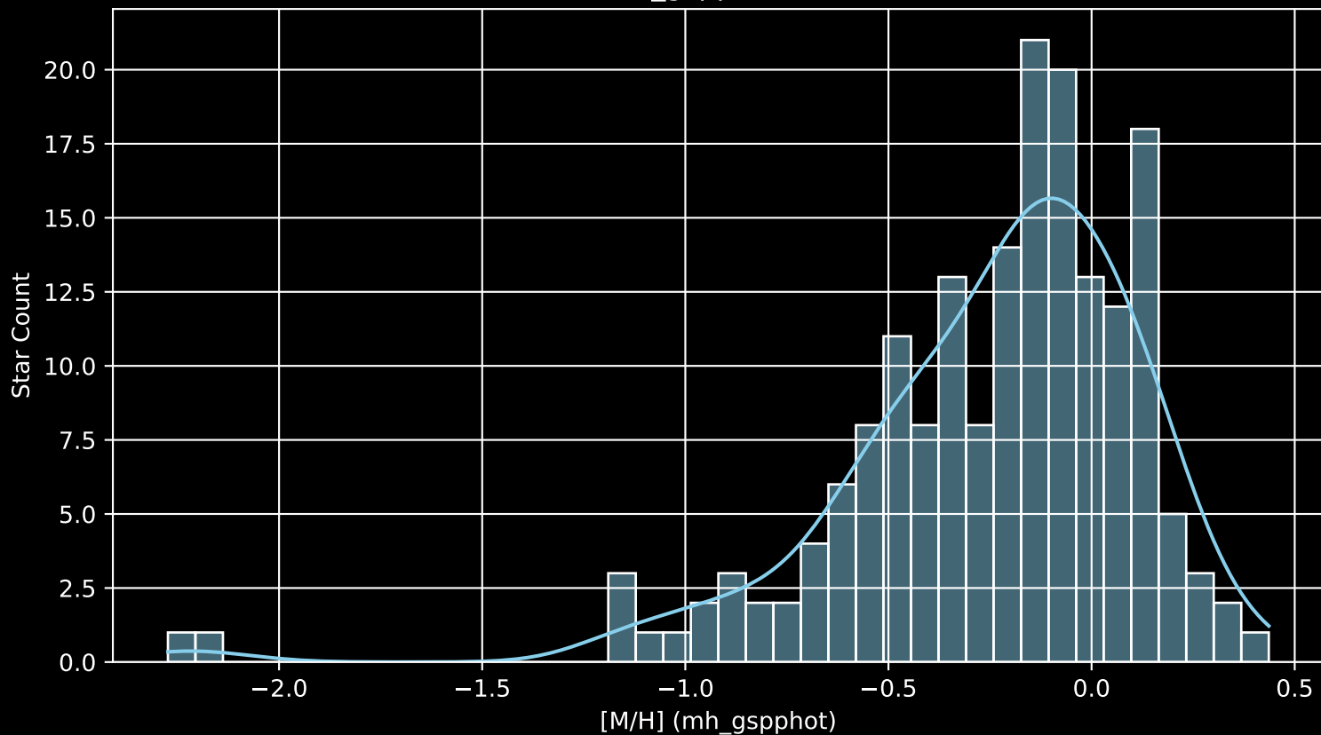
APOGEE DR17 Field: [K2_C7_010-14_btx [M/H] (mh_gspphot) (n= 183)
