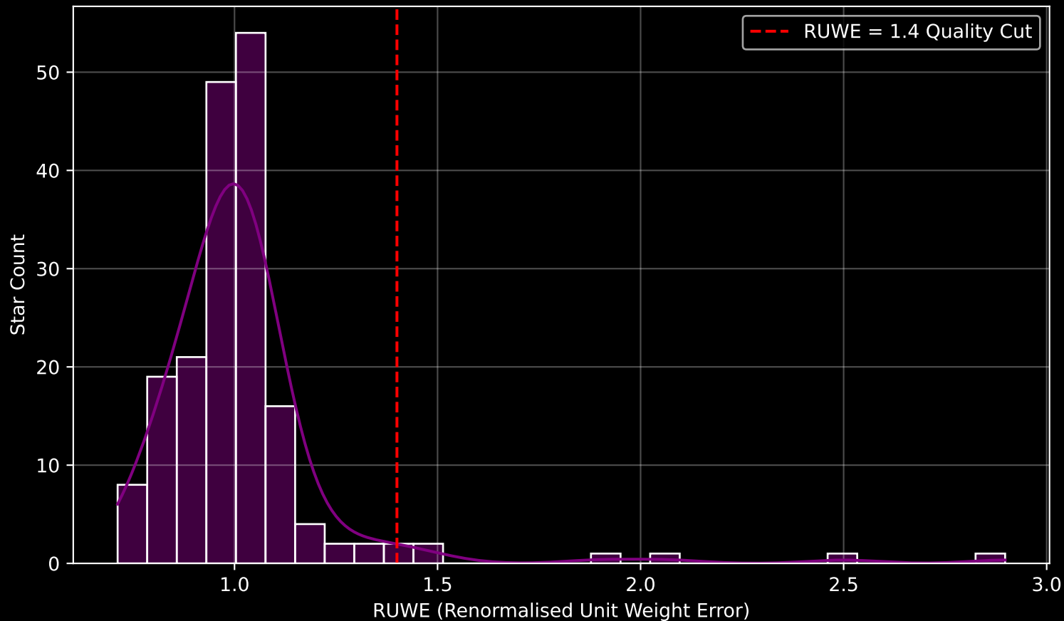
GAPOGEE DR17 Field [K2_C7_010-14_btx] RUWE Distribution (n= 183)
